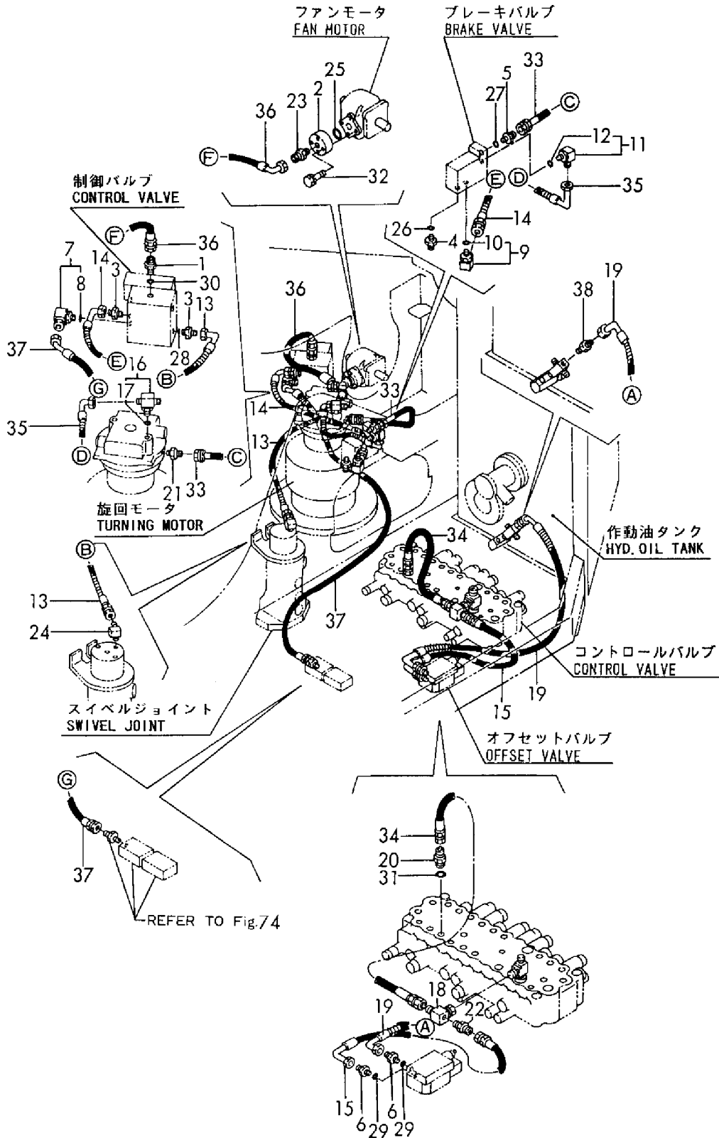
Fig. 69 油圧配管 HYD. OIL PIPING
